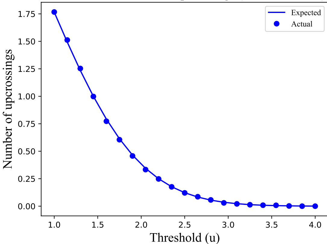
Validation for number of upcrossings (Gaussian fields)
