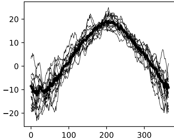
DataSample model
